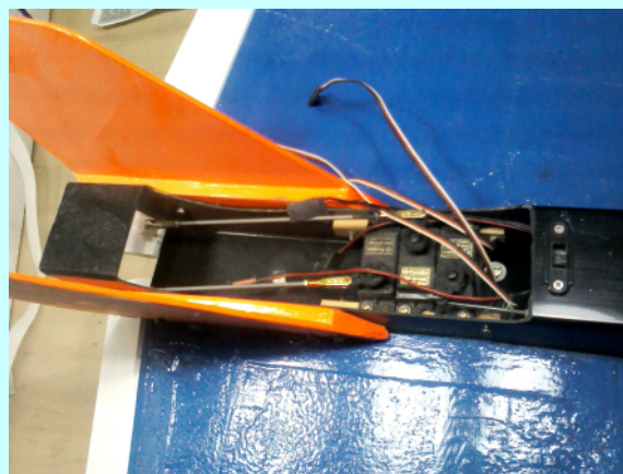
A nice simple radio installation. A template for the fuselage shape is available.
